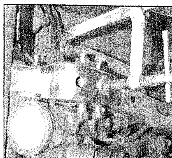
E. Bottom view showing proper alignment of steering box to the ART-135.
