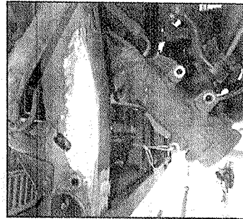
C. Factory steering box mount removed and frame rail ground down to bare metal.
