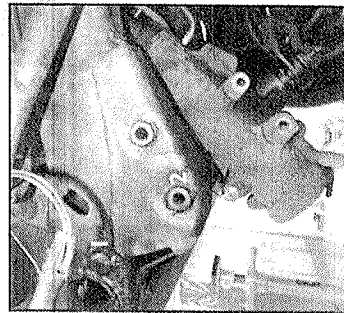
A. Factory steering box mount with steering box disconnected, 3 bolts hold it in place.
