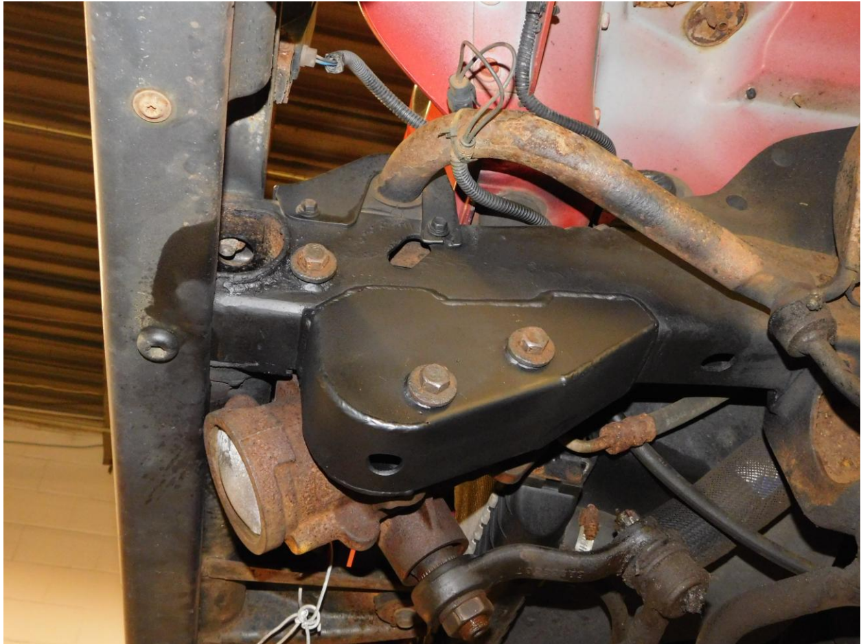
Illustration 10 new ART-135 with steering box bolted in place
